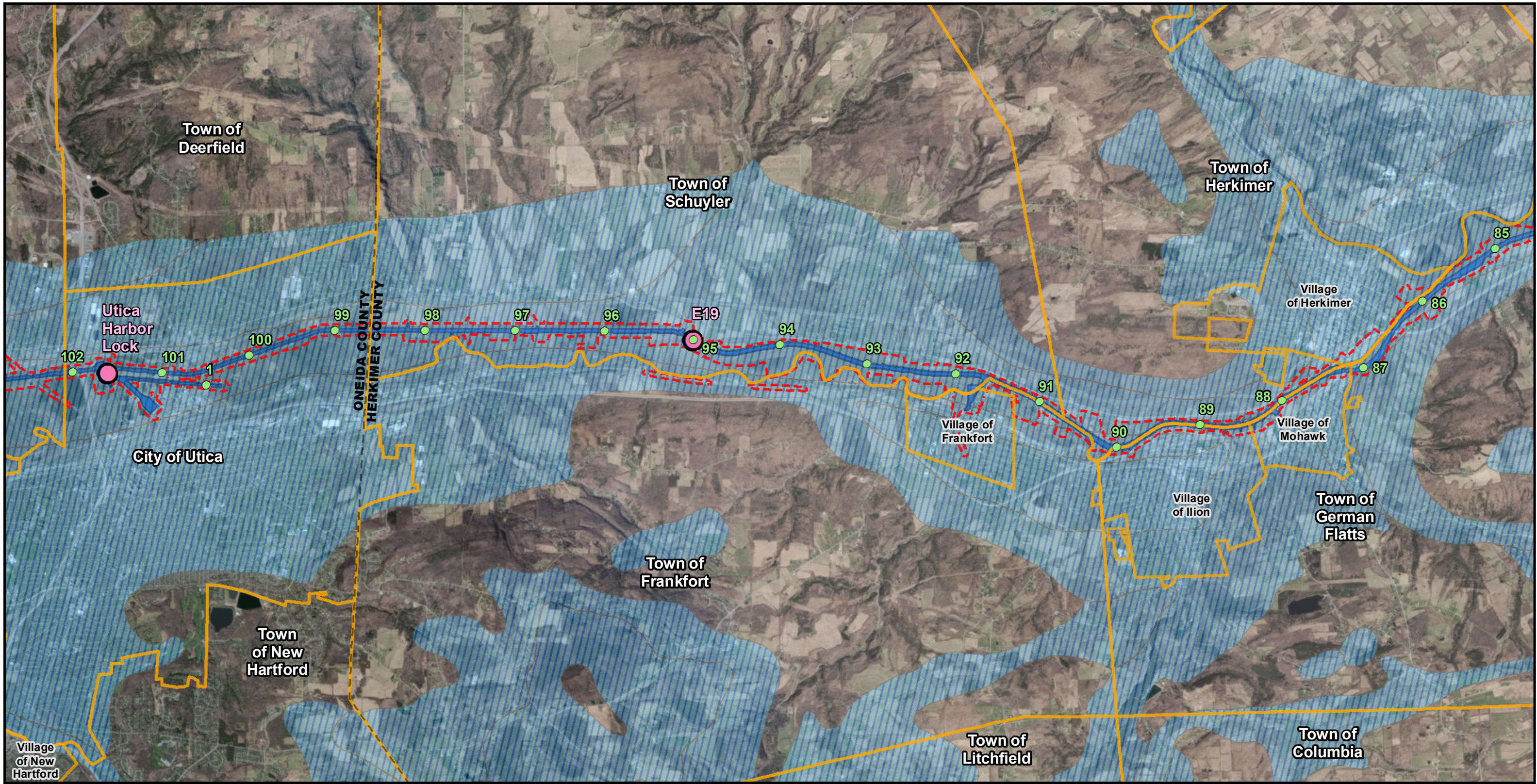
Figure 43F: Aquifers
